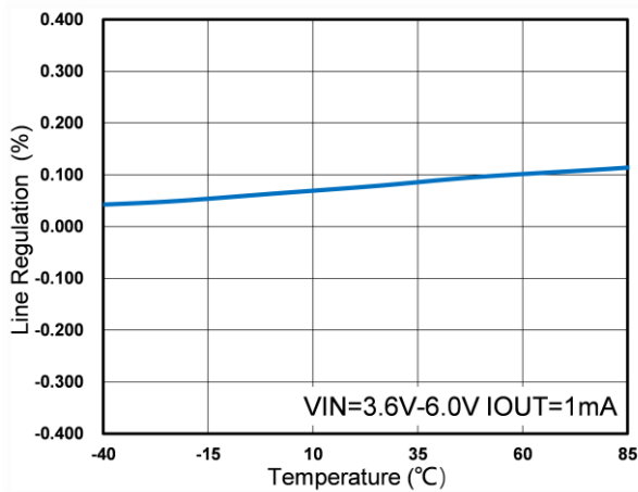
(9) Line Regulation VS Temperature
