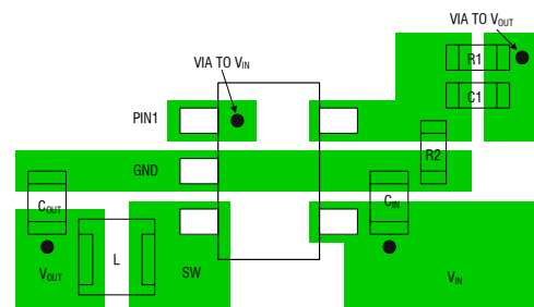
Figure 3. XR3406Suggested Layout
