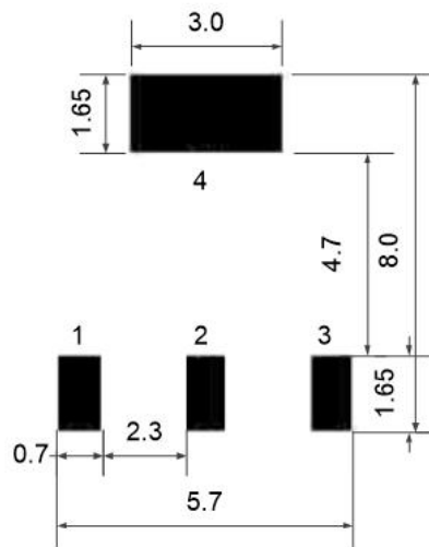
PCB Board
