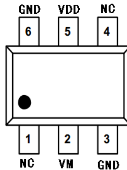
SOT23-6 TopView
