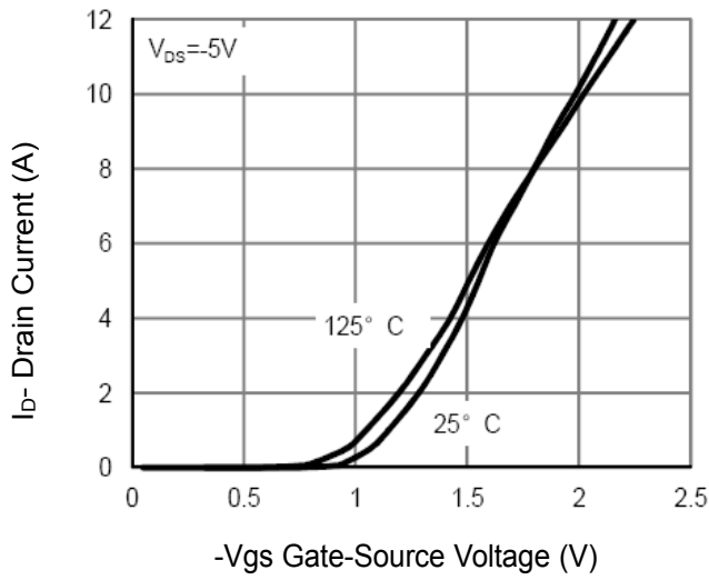
Figure 7 Transfer Characteristics
