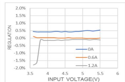
Line Regulation
