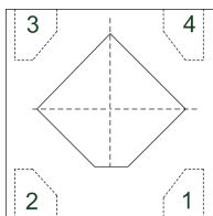
DFN1x1-4L (Top View)
