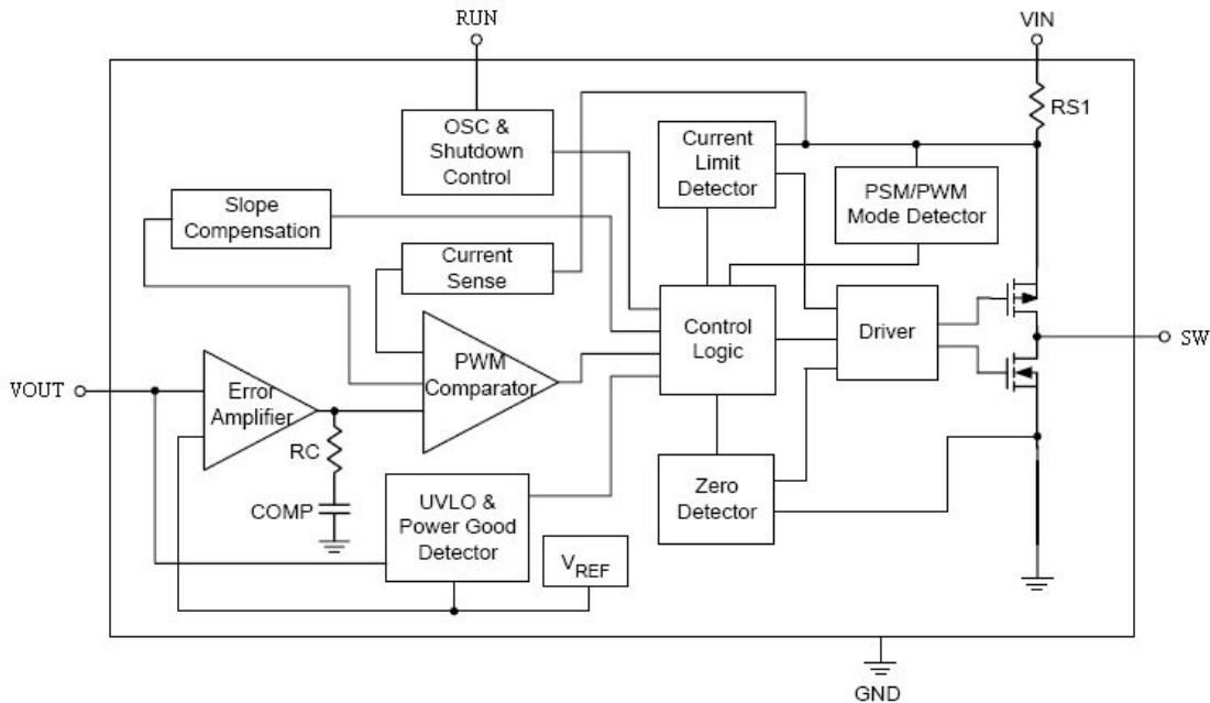
Figure 3. TC3488A Block Diagram
