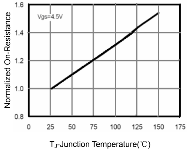
Figure 8 Drain-Source On-Resistance
